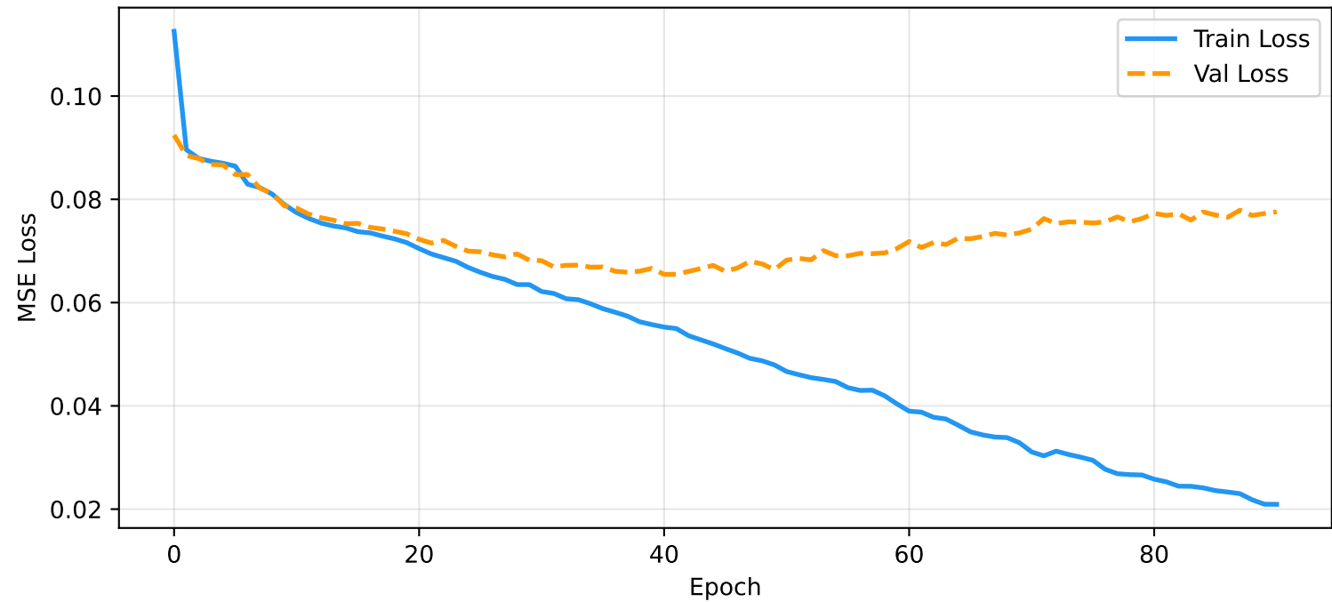
AutoEncoder - Training & Validation Loss
